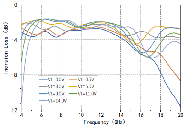
Insertion Loss VS Frequency @Pin=-10dBm
