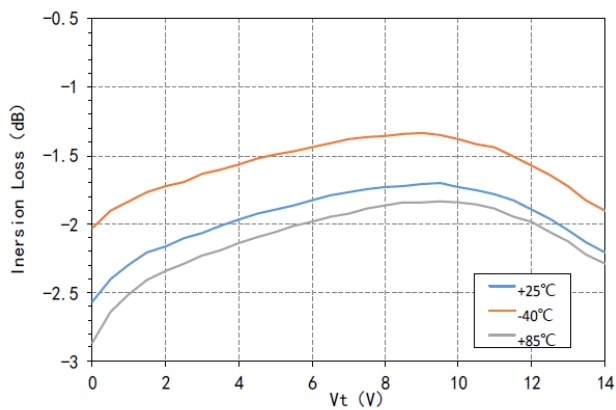
Insertion Loss VS V_t @12GHz
