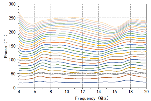
Phase VS Frequency@Pin=-10dBm ( V_t=0.5V \sim 14V )
